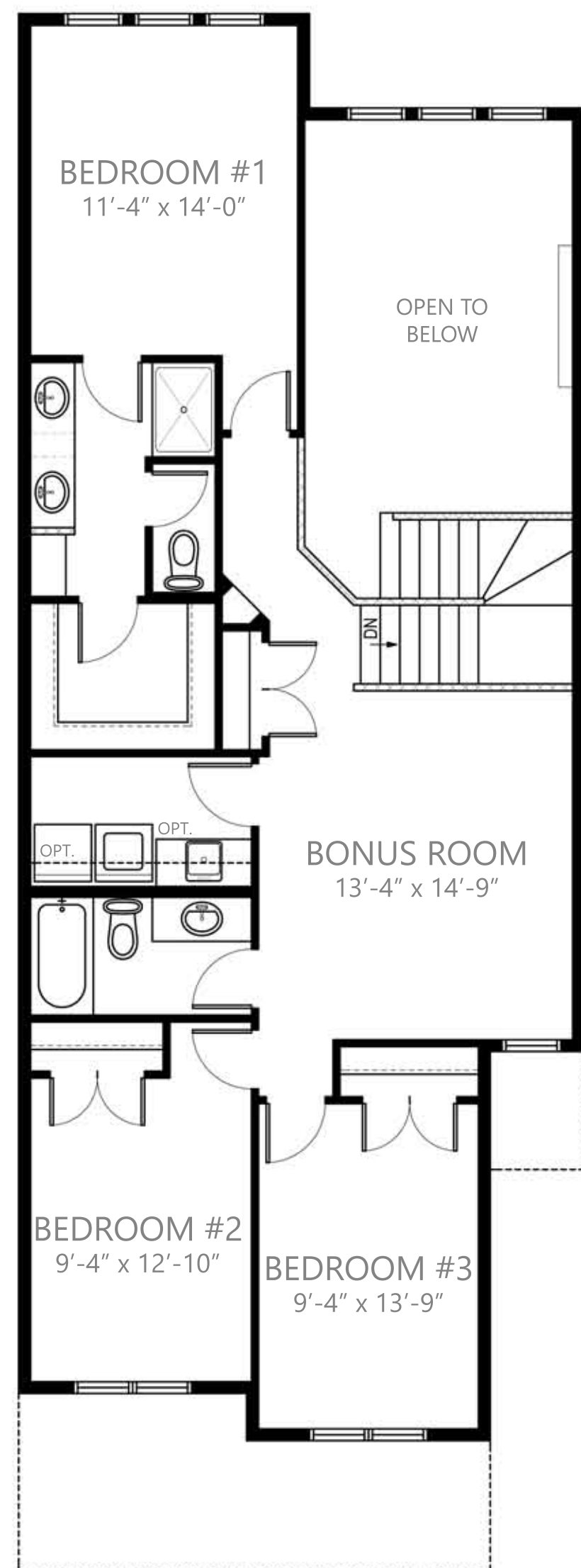
SECOND FLOOR - 1059 SQ.FT.
